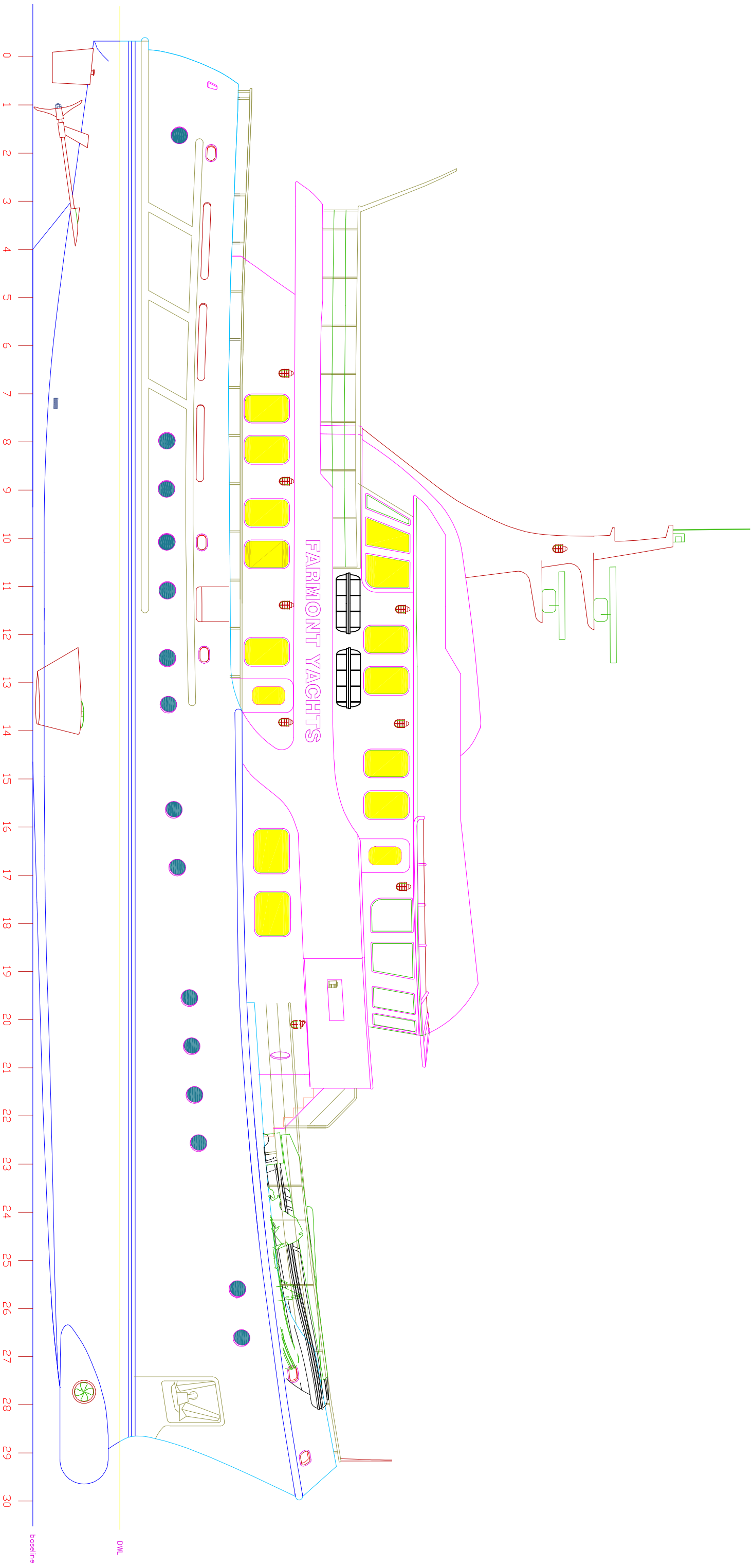
outboard profile
